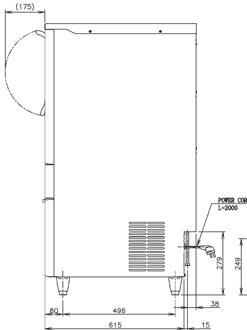
RIGHT SIDE
